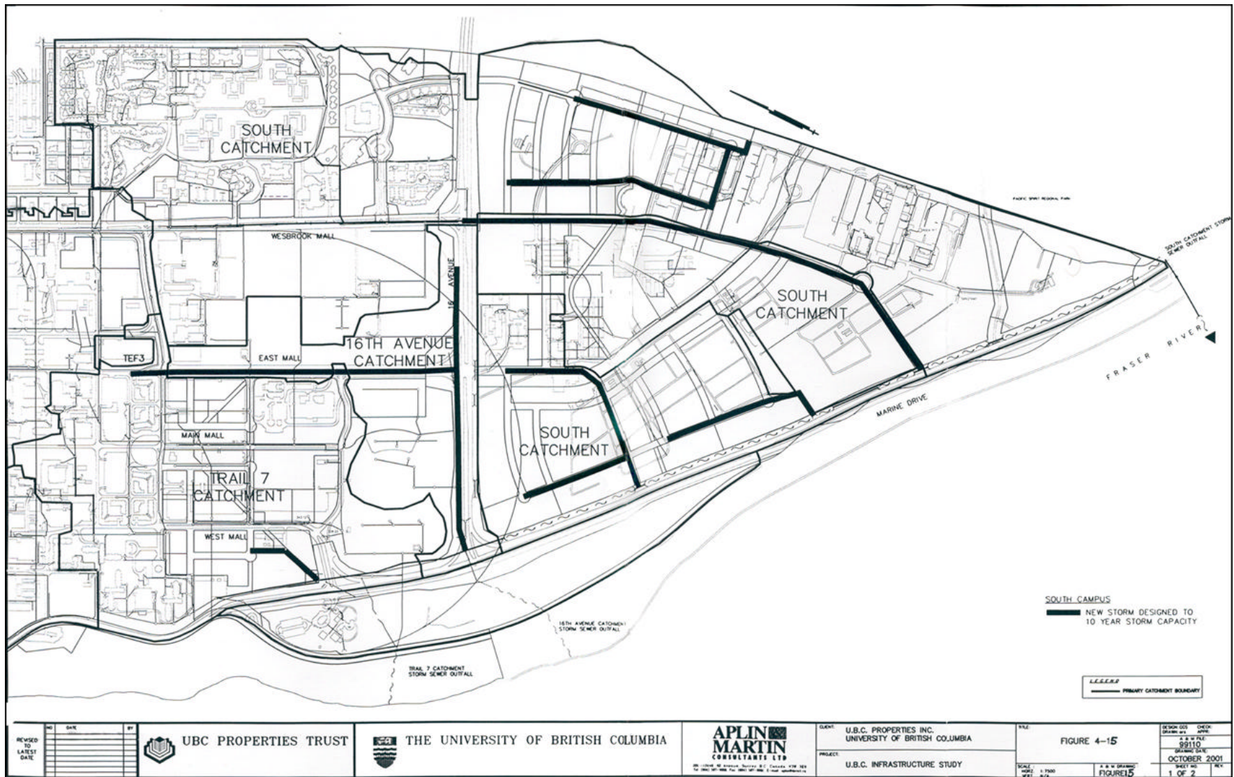
FIGURE 3.4 ALPIN & MARTIN 10-YEAR STORM INFRASTRUCTURE UPGRADE SYSTEM: SOUTH CAMPUS (ALPIN & MARTIN, 2001)
